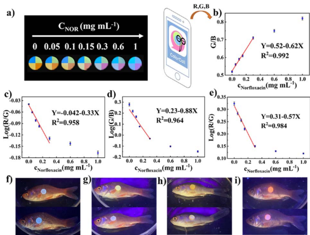
Fig. 5 (a) Photographs of color changes of four aliquots of COF BMTH-TFB , COF BMTH-TB , COF BMTH-TBT and COF BMTH-HB test strips after the addition of 4 μL NOR solution with different concentrations (0, 0.05, 0.1, 0.15, 0.3, 0.6 and 1 mg mL -1 from left to right, respectively). Fitted curves based on (b) COF BMTH-TFB , (c) COF BMTH-TB , (d) COF BMTH-TBT and (e) COF BMTH-HB using a smartphone to detect the NOR concentration via color change. Test paper based on (i) COF BMTH-TFB , (g) COF BMTH-TB , (h) COF BMTH-TBT and (f) COF BMTH-HB to detect fish scales before (top) and after (bottom) the addition of NOR.
