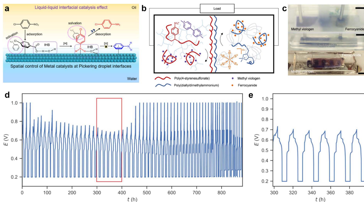
Fig. 8 (a) Schematic diagram of the reaction selectivity of p -CNB hydrogenation on the surfaces of Pd NPs, which is attached in the inner interface of Pickering droplets. IH-B is referred to as the interfacial hydrogen-bonding interaction. Reproduced with permission. 101 Copyright © 2023 American Chemical Society. (b) Mechanism of all liquid batteries based on structured-liquid. (c) Real picture of the all-liquid battery based on the biphasic system in cycling. Scale bars: 1 cm. (d) Full cell charge/discharge curves with long-term cycles for an under-oil all-liquid battery. (e) Cycles from 20th to 25th (marked by the red box in (d)). Reproduced with permission. 102 Copyright © 2022 American Chemical Society.
