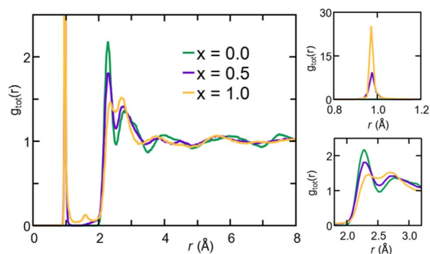
Fig. 3 (Color online) Left: Total pair correlation functions for amorphous \text{Na}_{3-x}\text{OH}_x\text{Cl} ( x = 0, x = 0.5 , and x = 1 ) obtained at T = 300 \text{ K} . Right: Zoomed-in view of the 0.8\text{--}1.2 (top) and 1.8\text{--}3.2 (bottom) ranges.
