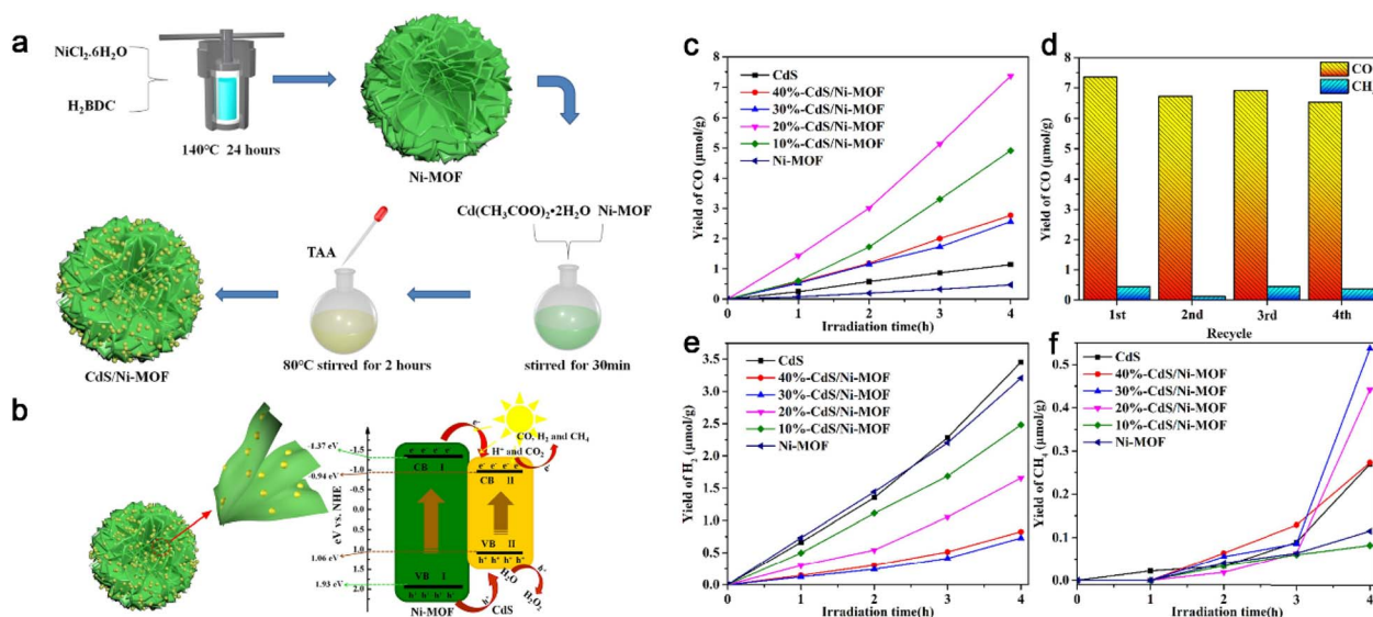
Fig. 28 (a) The schematic of the synthetic procedure of CdS/Ni-MOF. (b) The schematic of CdS/Ni-MOF for photocatalytic reduction of \text{CO}_2 . (c) CO yield; (d) repeat experiment diagram; (e and f) yields of \text{H}_2 and \text{CH}_4 . Reprinted with permission from ref. 221.
