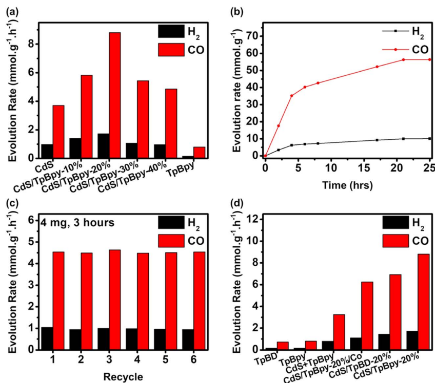
Fig. 4 (a) Influence of the amount of TpBpy integrated with CdS on the CO and \text{H}_2 evolution rates. (b) Product yield activity over time for CdS/TpBpy-20%. (c) Catalyst recycling experiments of the optimized nanohybrid. (d) Comparison of activities of various samples.
