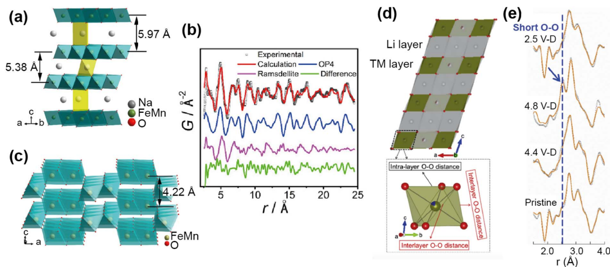
Fig. 11 (a) Structure of the OP4 phase. (b) Refined NPDP pattern of the desodiated sample, showing contributions from the OP4 phase and the ramsdellite phase. (c) Schematic illustration of the ramsdellite structure. Reprinted with permission from ref. 65 Copyright 2020 American Chemical Society. (d) Structure of \text{Li}_{1.2}\text{Ni}_{0.13}\text{Mn}_{0.54}\text{Co}_{0.13}\text{O}_2 and \text{TMO}_6 octahedra showing interlayer and intralayer O–O distance. (e) Comparison of the ex situ NPDP results of LMR-NMC collected at different charge–discharged states. Reprinted from ref. 66 Copyright (2020), with permission from Elsevier.
