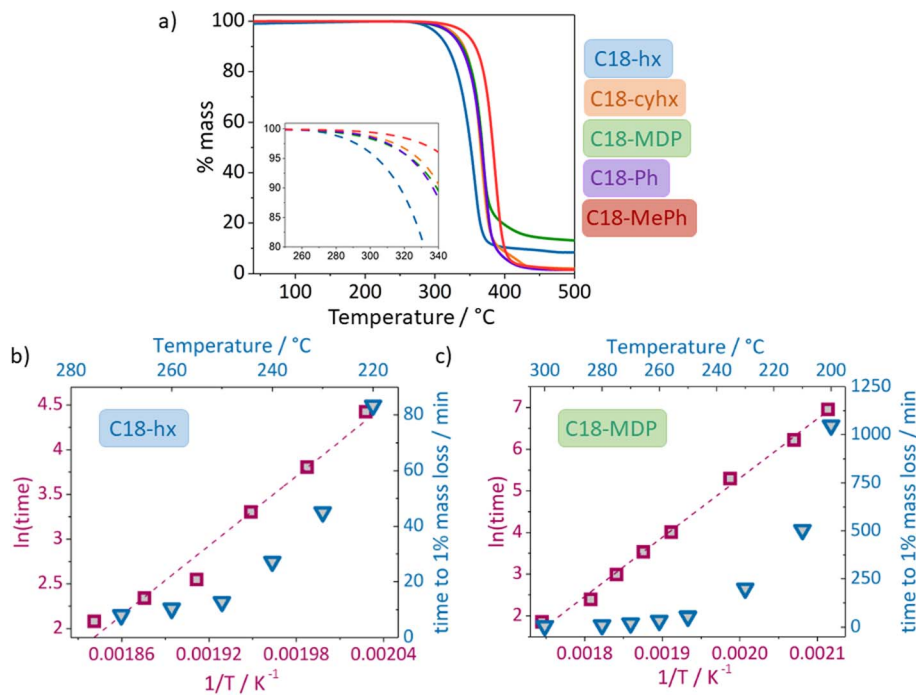
Fig. 6 (a) TGA curves of C18-hx, C18-cyxh, C18-MDP, C18-Ph and C18-MePh at a 10\text{ °C min}^{-1} heating rate. The inset shows the expanded temperature range where decomposition begins. (b) and (c) Show the isothermal TGA time taken for 1% mass loss to occur (top and right axes in blue) and Arrhenius plots of this data with linear fits (wine coloured axes and data points) for C18-hx and C18-MDP respectively.
