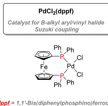
Fig. 11 Palladium–diphosphine complex used for Suzuki coupling.
