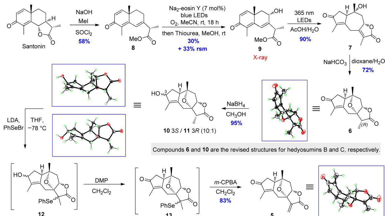
Scheme 3 Synthesis of key intermediate hedyosumin A (5). LED = light-emitting diode; RSM = recovered starting material; LDA = lithium diisopropylamide; Ph = phenyl; DMP = Dess–Martin periodinane; m -CPBA = meta -chloroperoxybenzoic acid.
