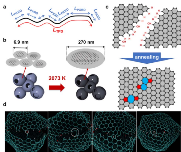
Fig. 4 (a) An illustration of and comparison of L_{PXRD} and L_{TPD} . (b) Evolution of the entire graphene size before and after 2073 K. (c) An illustration of zipping reaction of graphene domains. (d) Molecular dynamic simulation of the zipping reactions.
