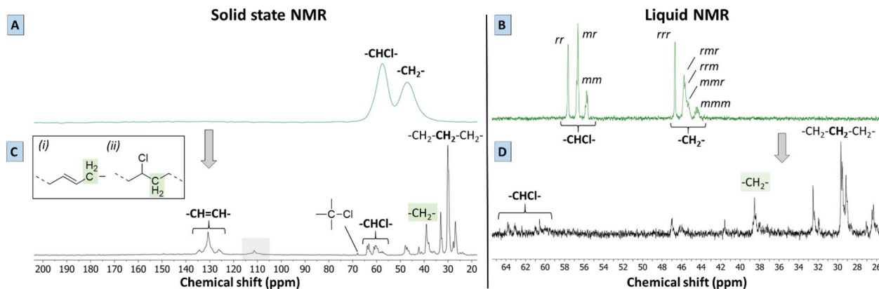
Fig. 5 Solid state (MAS) NMR spectra of PVC (A) and of the product (C) containing double bonds (130 ppm). In C, the signal at 110 ppm (grey box) is background signal from probe. Marked ‘-CH 2 -’ peaks comprise (i) allylic CH 2 , (ii) \alpha -CH 2 next to -CHCl- groups. Liquid 13 C NMR (d 8 -THF, 400 MHz) shows tacticity of PVC (B) and microstructure of polymer product (D). The product has 81% dechlorination and 7 double bonds per 100 C from tandem dehydrochlorination-hydrogenation (0.5 mol% H(CO)Rh(PPh 3 ) 3 , 0.85 mmol Bu 4 Pf 6 , 1 mL 2-butanone per 1 mmol PVC, 20 bar H 2 at 180 °C).
