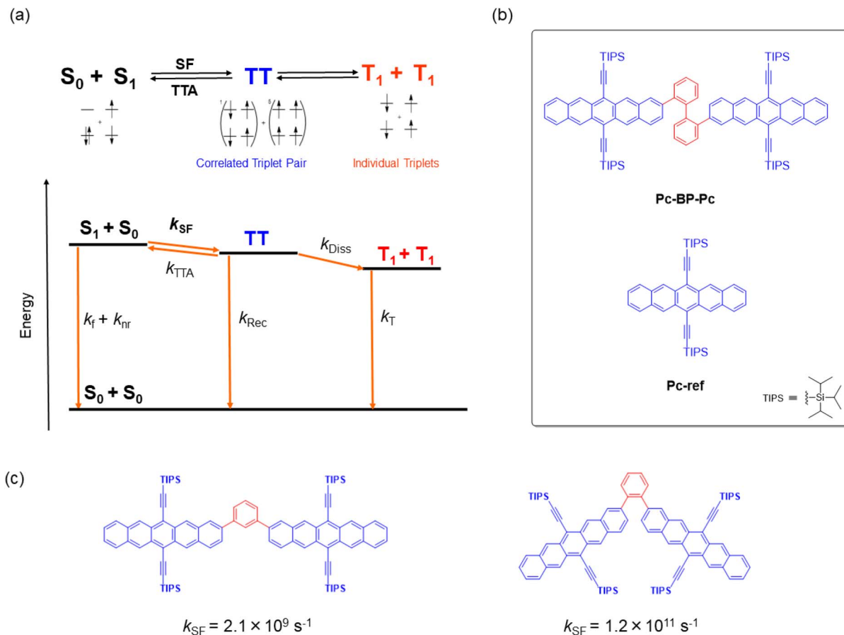
Fig. 1 (a) Schematic of the mechanism of SF in a TIPS-pentacene dimer. k_f and k_{nr} : deactivation processes from S_1 ; k_{SF} : SF from S_1 to TT; k_{TTA} : reverse triplet-triplet annihilation process from TT to S_0 + S_1 ; k_{Rec} : recombination process from TT to S_0 ; k_{Diss} : dissociation process from TT to T_1 + T_1 ( 2T_1 ); k_T : deactivation process from 2T_1 to S_0 . Considering the reported energies of S_1 (1.9 eV) and TT (1.6 eV), the reverse triplet-triplet annihilation process (TT \rightarrow S_0 + S_1 ) can be omitted because of the large exergonic trend ( \sim 0.3 eV). 42 (b) Target chemical structures of Pc-BP-Pc and Pc-ref . (c) Structures and their SF rates of TIPS-pentacene dimers that are linked by m - and o -phenylenes. 42
