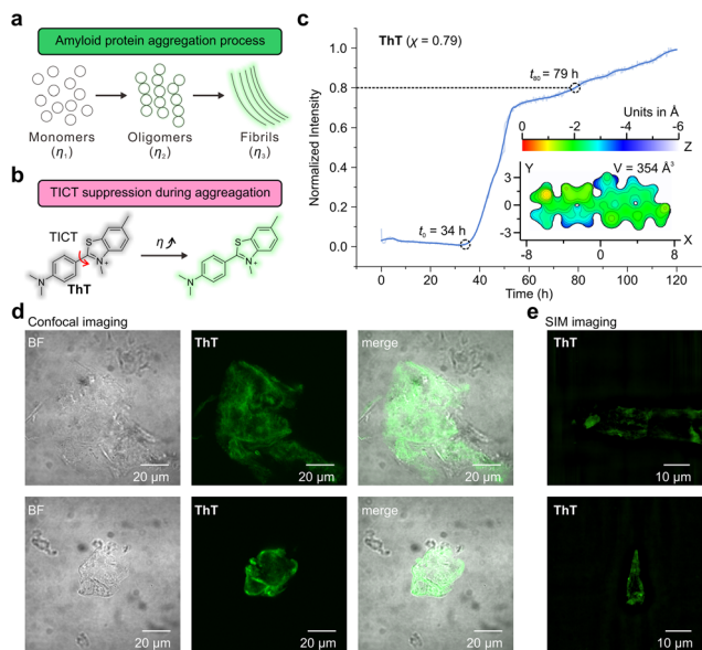
Fig. 5 (a) The illustration of the protein aggregation process. (b) The TICT-based sensing mechanism of Thioflavin T (ThT). (c) Normalized fluorescence intensity of ThT during the aggregation of \text{A}\beta proteins. (d) Confocal and (e) SIM fluorescence imaging of \text{A}\beta proteins using ThT. BF stands for the bright field. The two rows in (d) and (e) represent two selected regions of the sample chosen for imaging. The surface distance projection map and the volume of ThT are labelled in the inset.
