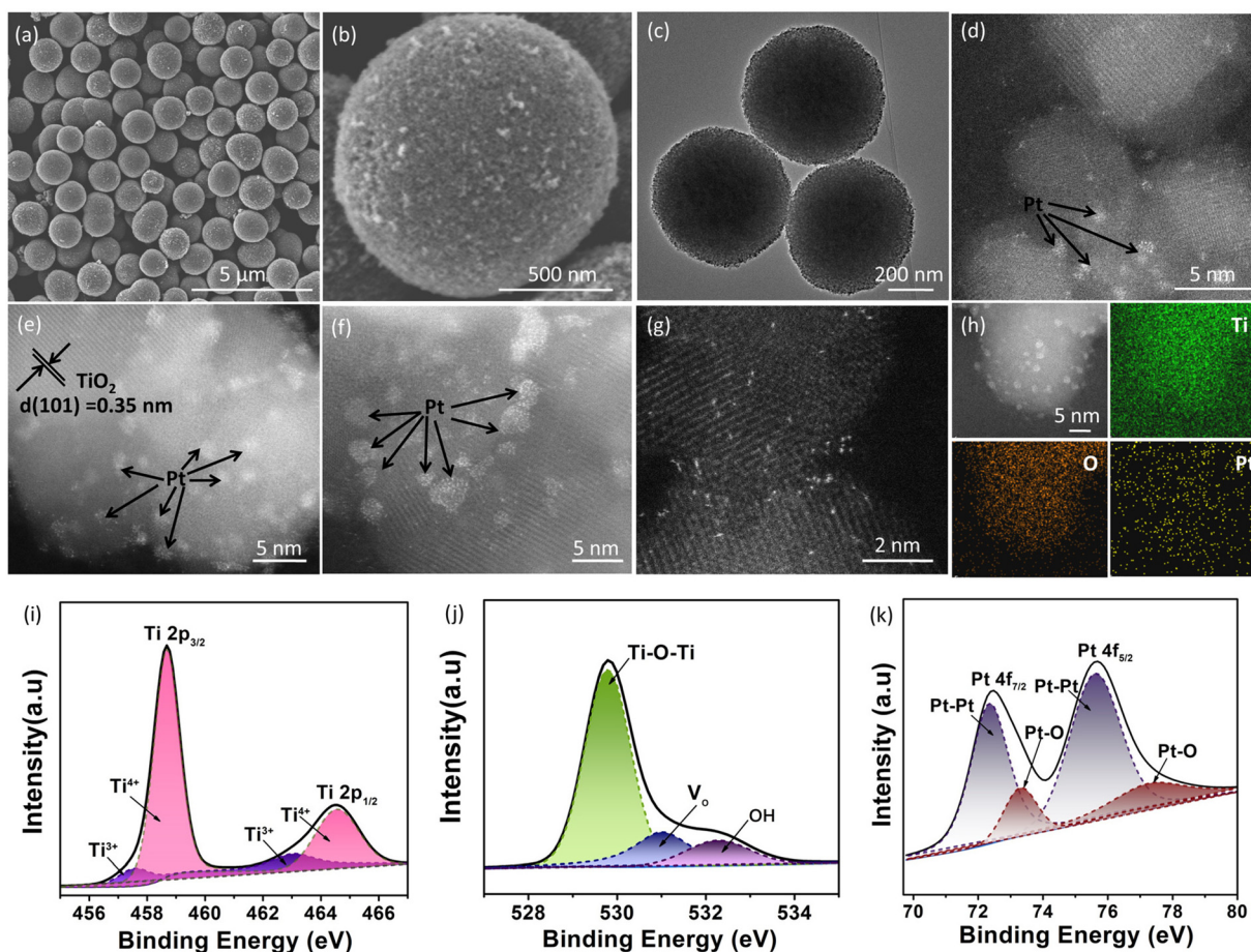
Fig. 2 (a and b) SEM and (c) TEM image of bare \text{TiO}_2 . (d–g) Spherical aberration-corrected HAADF-STEM image of 0.2% \text{Pt}/\text{TiO}_2 (d), 0.4% \text{Pt}/\text{TiO}_2 (e and g) and 1.0% \text{Pt}/\text{TiO}_2 (f). (h) HAADF-STEM and elemental mapping images of 0.4% \text{Pt}/\text{TiO}_2 . (i–k) High-resolution Ti 2p, O 1s and Pt 4f XPS spectra of 0.4% \text{Pt}/\text{TiO}_2 .
