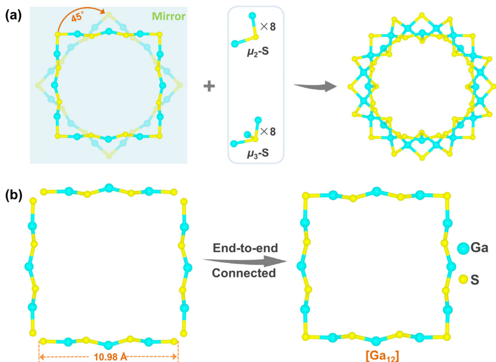
Fig. 2 (a) Mirror symmetric two [Ga 12 ] folded quasi-ideal square (coordinated CPA is omitted) linked together through 8 \mu_2 -S 2- and 8 \mu_3 -S 2- by twisting \sim 45^\circ to form the wheel-shaped molecular ring and (b) a [Ga 12 ] unit constructed by 4 1D polymeric chains of 3 Ga 3+ ions and 4 adjacent bridged \mu_2 -S 2- .
