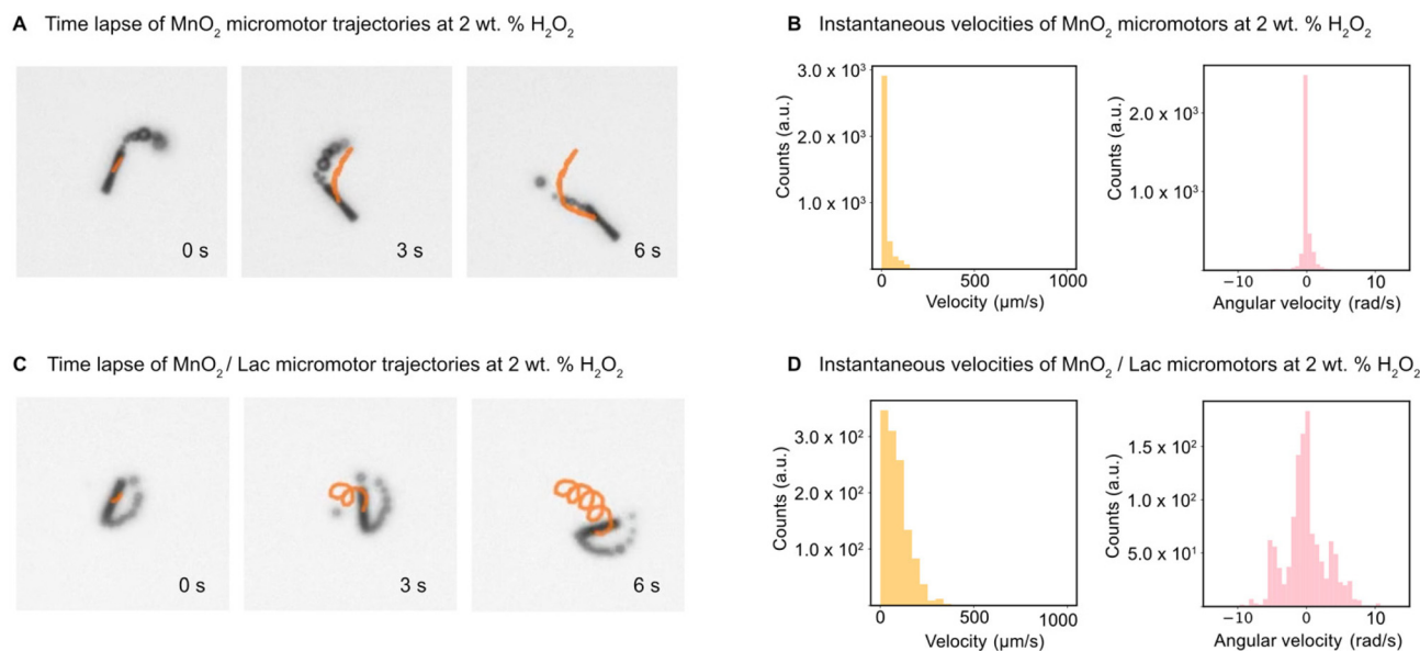
Fig. 5 Motion characterization of MnO 2 and MnO 2 /Lac micromotors at 2 wt% H 2 O 2 . (A) Time-lapse of MnO 2 micromotors trajectories. (B) Velocities and angular velocities for MnO 2 micromotors. (C) Time-lapse of MnO 2 /Lac micromotors trajectories. (D) Velocities and angular velocities for MnO 2 /Lac micromotors.
