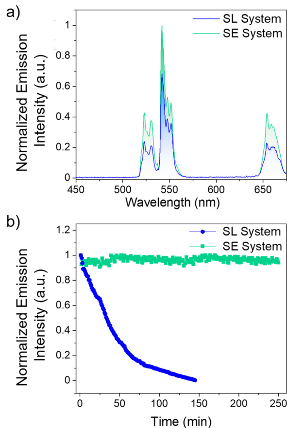
Fig. 3 (a) Normalized upconversion emission spectra of the SL and SE systems under 800 nm excitation. (b) Emission intensity of the {}^4\text{S}_{3/2} , {}^2\text{H}_{11/2} \rightarrow {}^4\text{I}_{15/2} transition of \text{Er}^{3+} in the SL (blue) and SE (green) systems as a function of time under 800 nm excitation.
