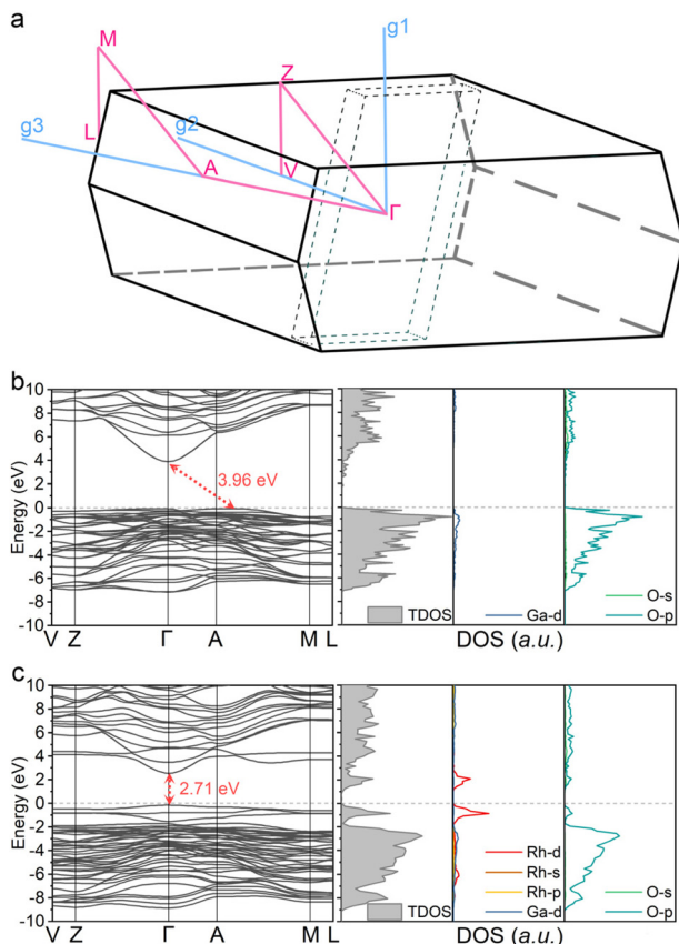
Fig. 3 (a) The high symmetry pathway of \beta -Ga 2 O 3 in the Brillouin zone. The K points are V = (0 \frac{1}{2} 0) , Z = (\frac{1}{2} \frac{1}{2} 0) , \Gamma = (000) , A = (0 \frac{1}{2} \frac{1}{2}) , M = (\frac{1}{2} \frac{1}{2} \frac{1}{2}) , L = (0 \frac{1}{2} \frac{1}{2}) . Band structures by HSE06, calculated TDOS and PDOS of (b) \beta -Ga 2 O 3 and (c) Rh doped \beta -Ga 2 O 3 . The top of the valence band is aligned to zero.
