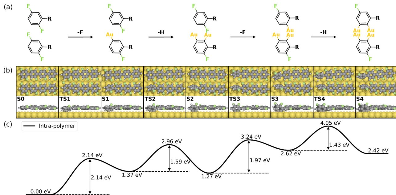
Fig. 3 Reaction mechanism of the first four steps of the HF zipping reactions (S0-S4). (a) The valence bond structure of each intermediate state. (b) The reaction pathway and (c) the corresponding energy profile. Definition of energies is given in eqn (S3) (see ESI†). The C, H, F, and Au atoms are represented by the gray, white, green, and yellow circles, respectively.
