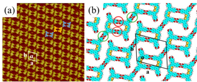
Fig. 1 (a) High-resolution STM image of H 4 BDETP's linear structure at the 1-heptanoic acid/HOPG interface, and the tunneling conditions were: I_{\text{set}} = 216.7 pA, V_{\text{bias}} = 707.4 mV ( 32.0 nm \times 32.0 nm). (b) The calculated molecular model for the linear structure.
