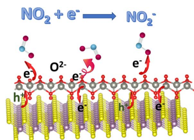
Fig. 3 NO 2 sensing mechanism based on an ionosorption model for 2D materials.
