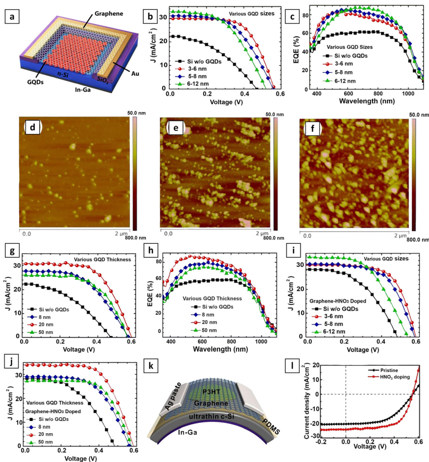
Fig. 7 (a) Schematic diagram of the GQDs/Si device with Gr thin film. (b) and (c) J - V characteristics and EQE spectra of GQDs/Si devices manufactured with GQDs of various sizes. (d)–(f) AFM micrograph of GQDs film with different thicknesses of 8, 20, and 50 nm. (g) and (h) J - V characteristics and EQE spectra of GQDs/Si devices manufactured with GQDs of various thicknesses. (i) and (j) J - V characteristics of the GQDs/Si solar cell after HNO 3 doping. Reproduced from ref. 113, with permission from Elsevier. (k) Schematic diagram of the flexible graphene/ultrathin c-Si solar cell. (l) J - V characteristics of solar cell with and without HNO 3 doping. Reproduced from ref. 114, with permission from the Royal Society of Chemistry.
