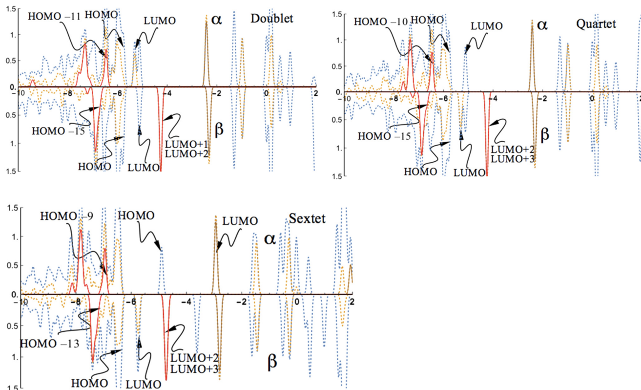
Fig. 7 PDOS of the \text{Ni}_I substituted (111)_n surface phase of \gamma\text{-Al}_2\text{O}_3 in the doublet, quartet, and sextet states. The surface layer consists of one \text{Ni}_I atom, two Al atoms, and twelve O atoms ( \text{Ni}_I , \text{Al}_I , \text{Al}_{II} , \text{O}_n , n = 1 to 12; see Fig. 1). The dotted blue lines are from both \text{Ni}_I substituted and unsubstituted surface layers; the dotted orange lines are the contribution from the \text{Ni}_I substituted surface layer; the solid red lines are the contribution from d-type orbitals of \text{Ni}_I ; the solid brown lines are the contribution from s-type orbitals of \text{Ni}_I .
