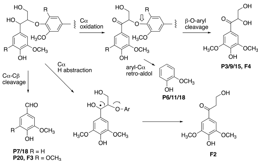
Fig. 10 Formation of products from polymeric lignin. R = H (guaiacyl G lignin unit) or \text{OCH}_3 (syringyl S lignin unit). Further oxidation of vanillin (P7/18) generates the corresponding carboxylic acid, vanillic acid (P2). Poplar organosolv lignin contains both S and G units (with proportion of S > G).
