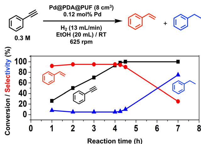
Fig. 5 Hydrogenation of phenylacetylene with Pd@PDA@PUF ( 8 \text{ cm}^3 ); black squares: PA conversion; red circles, ST selectivity; blue triangles: EB selectivity. Reaction conditions: PA ( 6 \text{ mmol} ), Pd ( 7 \times 10^{-3} \text{ mmol} , 0.12 \text{ mol}\% ), EtOH ( 20 \text{ mL} ), \text{H}_2 flow rate ( 13 \text{ mL min}^{-1} ), room temperature, 625 \text{ rpm} .
