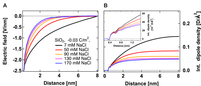
Fig. 2 Electric field E_z (A) and integrated dipole density (B) as a function of z -distance from the surface from simulations with a constant surface charge density of -0.03 \text{ C m}^{-2} but at different ionic concentrations. The electric field is calculated only from ionic and \text{SiO}_2 charges, i.e. , without the contribution from water molecules. The dipole density is the product of the number density of water molecules, the cosine of the angle between the surface normal and water dipole, and the dipole moment of the SPC/E water model equal to 2.35 D.
