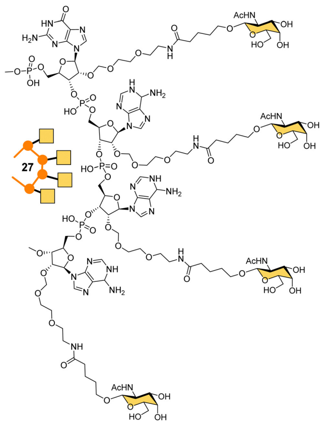
Fig. 10 The chemical structure of GalXC with a tetraivalent hairpin loop developed by Dicerna Pharmaceuticals.
