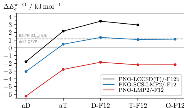
Fig. 9 Comparison of PNO (with aX≡aVXZ) and PNO-F12 (with X-F12≡VXZ-F12) predictions of the relative electronic stabilities of c2NA O and c2NA π (ΔE e π-O ) for increased coverage of the one-particle basis space. The optimised B3LYP-D3 abc (BJ)/def2-QZVP geometries are used (reference values shown in grey).
