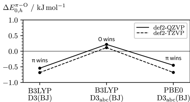
Fig. 8 Impact of the basis size, exchange–correlation functional, and inclusion of three-body dispersion on the relative stabilities of c2NA O and c2NA π (ΔE 0,h π-O ).
