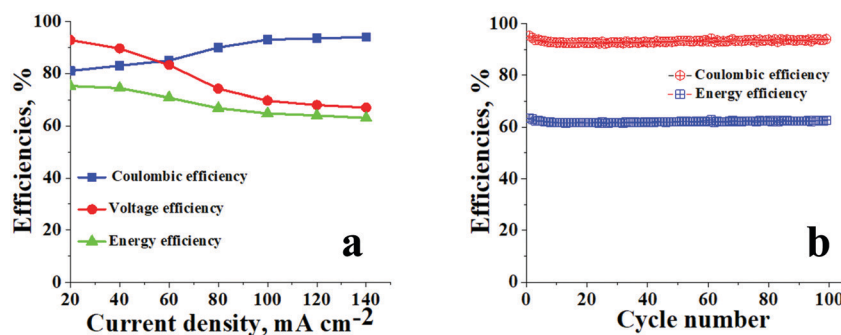
Fig. 5 Battery performance of ICEM. (a) CEs, VEs and EEs of ICEM at different current densities; (b) CEs and EEs of ICEM at 140 mA cm -2 over 100 cycles.
