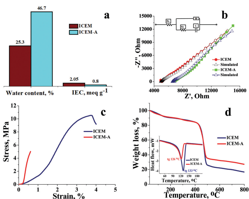
Fig. 3 Comparative physicochemical and mechanical analysis of ICEM and ICEM-A. (a) Water content and IEC. (b) Impedance spectra with simulation with the circuit diagram as the inset figure. (c) Mechanical strength analysis and (d) TGA spectra with the inset image showing the DSC spectra.
