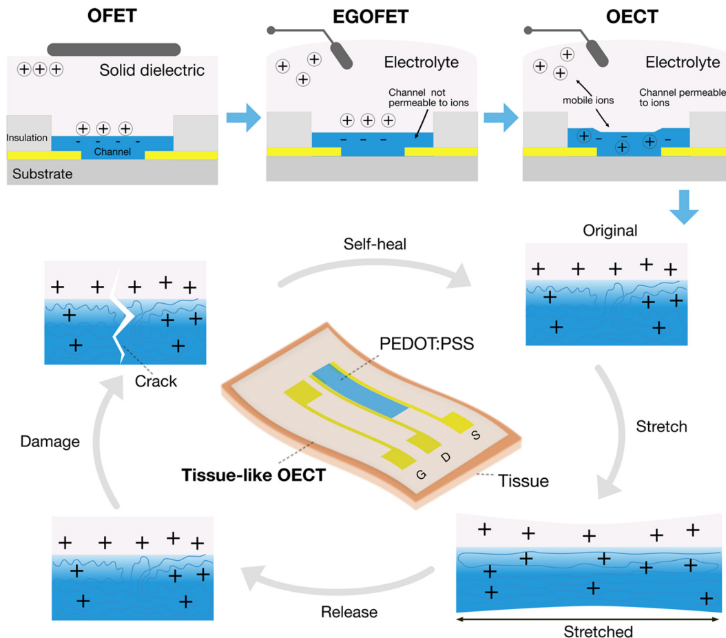
Fig. 1 Schematic of an OFET, EGOFT, OEFT and tissue-like OEFTs.
