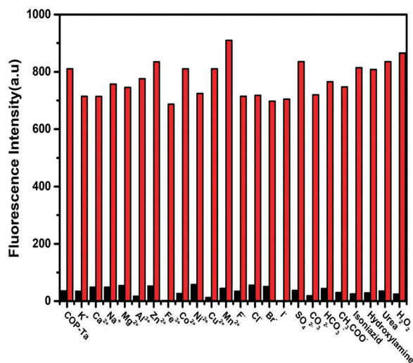
Fig. 5 Comparison of the fluorescence intensity of COP-Ta in the presence of various interfering components (100 \mu M) in water before (black bar) and after (red bar) the addition of hydrazine (200 mM).
