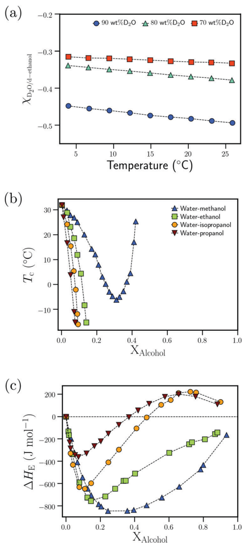
Fig. 8 Attractive interactions in the bulk solvent-cosolvent mixture: (a) dependence of the Flory-Huggins interaction parameter, \chi_{D2O-d-ethanol} , on the temperature for different D_2O wt% from ref. 111 (b) Dependence of the cloud point temperature, T_c , on the alcohol molar fraction, X_{Alcohol} , for different PNIPAM/water/alcohol mixtures from ref. 97 (c) Dependence of the excess enthalpy of mixing, \Delta H_E , on the alcohol molar fraction, X_{Alcohol} , for different water/alcohol mixtures as measured at 25 ^{\circ}C from ref. 112 Data in (a) has been reprinted (adapted) from ref. 111 Copyright 2016. Reproduced with permission from The American Chemical Society. Data in (c) has been reprinted (adapted) from ref. 112 Copyright 1965. Reproduced with permission from The American Chemical Society.
