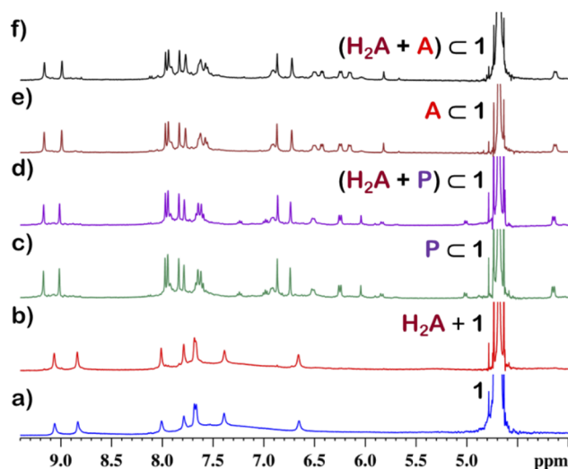
Fig. 6 Partial ^1\text{H} NMR stack plot of (a) 1 , (b) (\text{H}_2\text{A} + \mathbf{1}) ( \text{H}_2\text{A} = 9,10 -dihydroanthracene), (c) \text{P} < \mathbf{1} (P: phenanthrene), (d) (\text{H}_2\text{A} + \text{P}) < \mathbf{1} , (e) \text{A} < \mathbf{1} (A: anthracene) and (f) (\text{H}_2\text{A} + \text{A}) < \mathbf{1} in \text{D}_2\text{O} showing the selective encapsulation of A and P.
