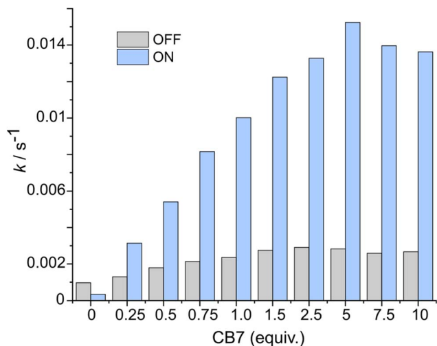
Fig. 3 Comparison of the rates of the hydrazone of the axle (75 \mu\text{M} ) at different amounts of CB7 in the dark (grey bars) and under constant light irradiation (blue bars), acetonitrile/ \text{H}_2\text{O} mixture ( v/v \approx 40 : 60 ), \text{pH} \approx 3 , 298 K. The determination of the rates is described in pp. S34–S35, ESI†
