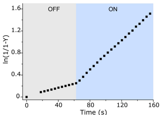
Fig. 4 Acceleration of the hydrazone reaction under constant light irradiation (blue region) after the initial \approx 60 s stay of the system (100 \mu\text{M} ) in the dark (grey region), acetonitrile/ \text{H}_2\text{O} mixture ( v/v \approx 40 : 60 ), \text{pH} \approx 3 , 298 K. Note that Y stands for the product yield, and the first datapoint in the blue region corresponds to the steady state of the photoswitch.
