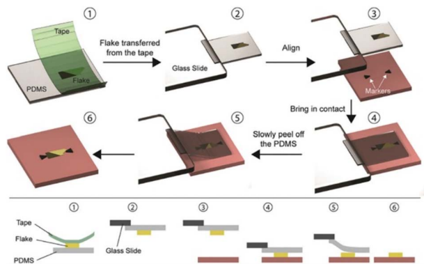
Fig. 3 The PDMS dry transfer method. The flake to be transferred is exfoliated onto a PDMS stamp (1) and the stamp is then attached to a glass slide connected to a micromanipulator (2). Using a microscope, the flake can be aligned with the final substrate (3) and brought into contact (4). By slowly peeling the PDMS stamp (5) the flake can be deposited on the substrate (6). Reproduced from ref. 81 with permission from Royal Society of Chemistry (RSC), copyright 2020.
