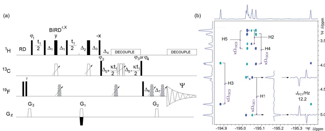
Fig. 6 (a) Pulse sequence of the (3, 2)D ^1\text{H}^n\text{C}^n\text{F} correlation experiment. For explanation of symbols used for pulses see Experimental. The NMR parameters used are given in Table S1.† The delays were as follows: d_2 = 0.25/{}^1J_{\text{HC}} ; d_3 = 0.5/{}^1J_{\text{HC}} ; d_4 = 0.25/{}^nJ_{\text{FC}} ; d_6 = \text{cnst}1/{}^1J_{\text{HC}} , where \text{cnst}1 = 0.5 for CH and 0.25 for \text{CH}_2 groups; \Delta_1 = d_3 - p14/2 ; \Delta_2 = d_2 - p14/2 - p16 - d16 ; \Delta_3 = d_2 - p14/2 - 2t_1(0) ; \Delta_4 = d_6 ; \Delta_5 = d_4 ; \Delta_6 = p16 + d16 - (2/\pi)p1 + 4 \mu\text{s} ; \Delta_7 = p16 + d16 + 4 \mu\text{s} , where p16 and d16 are the PFG length and the recovery time, respectively. The gradient strengths were as follows: G_1 = 40\% ; G_2 = 42.51\% ; G_3 = 13\% . The following phase cycling was used: \varphi_1 = y, -y ; \varphi_2 = 4x, 4(-x) ; \varphi_3 = 2x, 2(-x) ; \varphi_4 = 2y, 2(-y) ; \Psi = x, 2(-x), x, -x, 2x, -x . The echo-antiecho protocol was used with G_1 changing sign between real and imaginary increments. Phases \varphi_1 and \Psi were incremented by 180^\circ together with the sign change. Two interleaved experiments were acquired applying either the \varphi_3 or \varphi_4 phase to the last 90^\circ ^{13}\text{C} pulse, (b) an F_1 antiphase (3, 2)D ^1\text{H}^n\text{C}^n\text{F} spectra of 1 acquired using the pulse sequence shown in (a) showing the cross peaks of the \beta -anomer of 1 . Positive and negative cross peaks are shown in blue and turquoise, respectively. The insets contain vertical and horizontal traces through the H1, F cross peaks. The ^1\text{H} chemical shift of protons directly attached to ^{13}\text{C} atoms and the associated \kappa\Omega_{^{13}\text{C}} frequencies are indicated. Antiphase doublets in F_2 show ^nJ_{\text{FC}} coupling constants. Horizontal and vertical internal projections are shown on the top and along the left side of all spectra, respectively. The editing process that simplifies this spectrum is explained in the text and shown in Fig. S5.†
