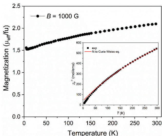
Fig. 1 Magnetic properties of \text{Na}[\text{o}^{57}\text{FESAN}] powder sample: temperature dependence of the magnetization under a magnetic field of 0.1 T. Inset: temperature dependence of the inverse of the magnetic susceptibility. The solid red line is the fit to the Curie–Weiss law of the experimental data (solid square symbols).
