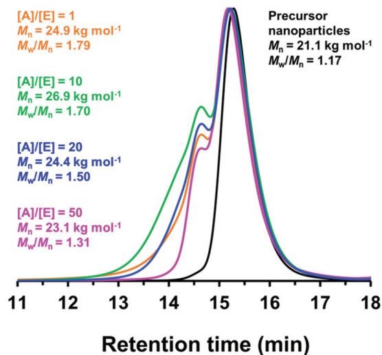
Fig. 3 GPC curves (vs. a series of near-monodisperse poly(methyl methacrylate) calibration standards) recorded using a refractive index detector for P(LMA 50 - stat -GlyMA 9 )-PMMA 67 (prepared in mineral oil at 20% w/w solids at 90 °C) (black curve) and the benzylamine-derivatized P(LMA 50 - stat -GlyMA 9 )-PMMA 67 produced when using an [amine]/[epoxy] molar ratio of 1 (orange curve), 10 (green curve), 20 (blue curve) or 50 (pink curve). A systematic reduction in M_w/M_n was observed when increasing the [amine]/[epoxy] molar ratio.
