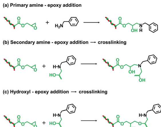
Scheme 2 Summary of the three possible reactions that can occur when reacting P(LMA 50 - stat -GlyMA 9 )-PMMA 67 nanoparticles with benzylamine. (a) Epoxy ring-opening results in the formation of a secondary amine and a hydroxyl group. (b) This secondary amine can then react with remaining epoxy groups. (c) Alternatively, the hydroxyl group can react with epoxy groups. Side-reactions (b) and (c) can lead crosslinking between and/or within stabilizer chains. In practice, the rate of reaction for (c) is expected to be slower than for (b).
