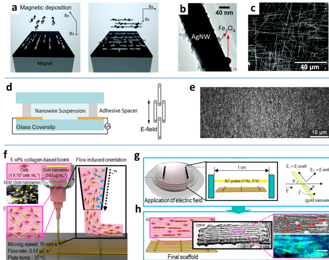
Fig. 9 (a) Illustration of the alignment of Fe_3O_4 -AgNWs in the magnetic field. (b) TEM image of the Fe_3O_4 -AgNW. (c) SEM image of the bi-aligned Fe_3O_4 -AgNWs. Reproduced with permission. 63 Copyright 2015, RSC Pub. (d) Schematic of the electric field-induced assembly of AuNWs. (e) Reflected light OM image of AuNWs. Reproduced with permission. 194 Copyright 2016, WILEY-VCH. (f) Schematic of the cell-printing process. (g) Schematic of the applied electric field for aligning AuNWs. (h) Schematic and optical/fluorescence images of the cell-laden collagen/aligned AuNW structure. Reproduced with permission. 84 Copyright 2019, American Chemical Society.
