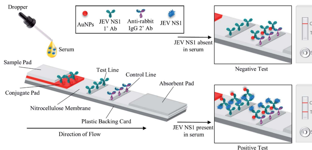
Fig. 1 The fabricated LFA strip consists of a plastic backing card with overlapping membranes, a porous nitrocellulose membrane coated with the JEV NS1 Ab and anti-rabbit IgG 2° Ab on test and control lines respectively, a conjugate pad with the AuNPs–JEV NS1 Ab conjugate, and a pre-treated sample pad at one end and an absorbent pad at the other end. In the case of negative samples, only the control line develops, whereas in the case of positive samples, both test and control lines develop.
