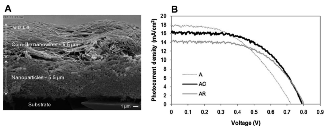
Fig. 8 (a) FE-SEM image of the cross sectional view of a double-layer film containing \text{TiO}_2 nanoparticles as the under-layer and corn-like \text{TiO}_2 nanowires as the over-layer. (b) Photocurrent density–voltage curves of fabricated \text{TiO}_2 solar cells [A- \text{TiO}_2 NP solar cell, AC- Corn like \text{TiO}_2 NW solar cell, AR-Regular \text{TiO}_2 NW solar cell]. 129 (Reprinted with permission from ref. Bakhshayesh, A. et al. , 2013. Copyright 2012 Elsevier Ltd.)
