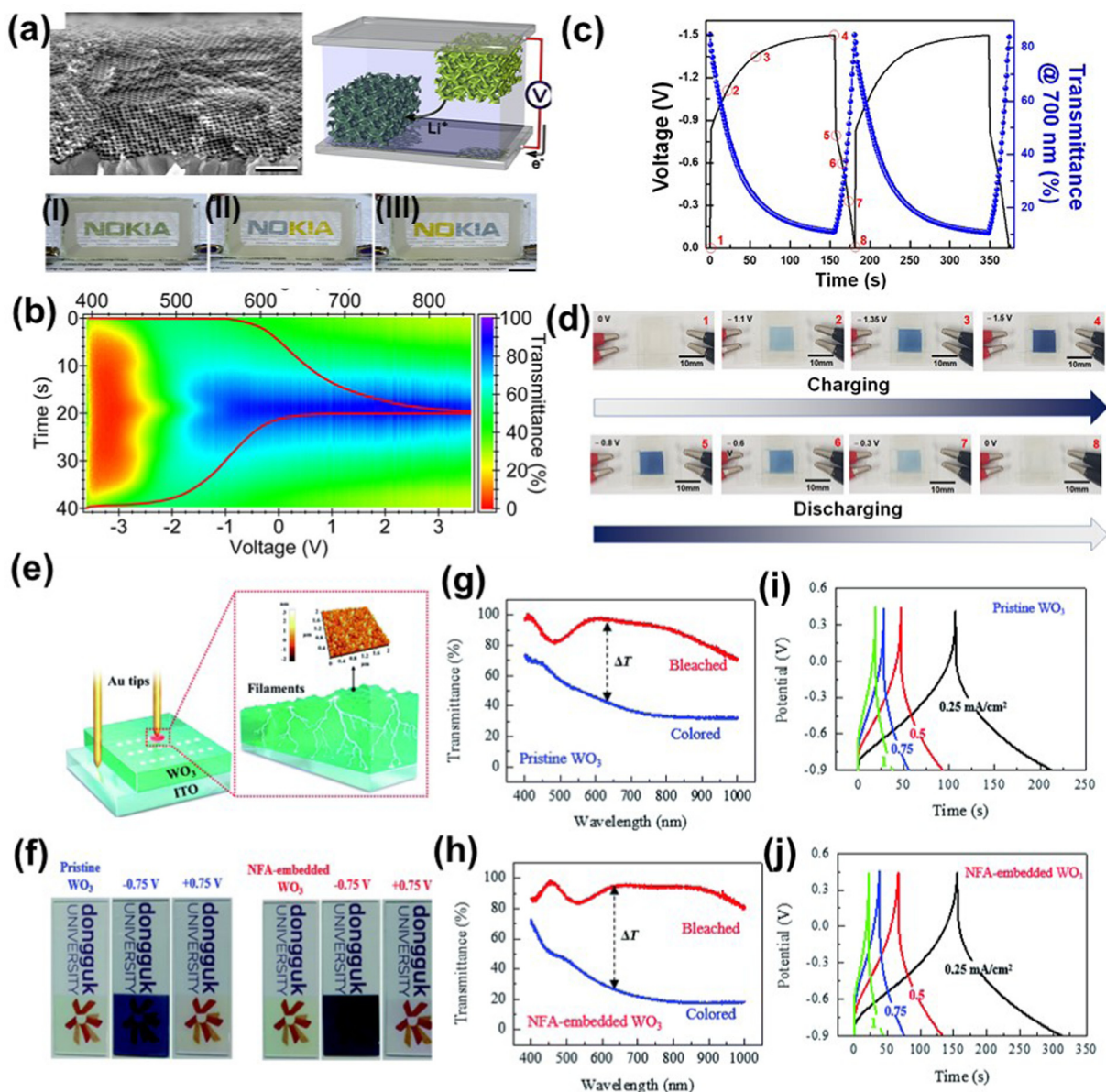
Fig. 6 SEM image of mesoporous V 2 O 5 double-gyroid structure (a), device structure of symmetric electrodes (all), and different optical images with "NO" and "KIA" (all). Transmittance variation during chronopotentiometry with alternating current polarity ( \pm 2 \text{ mA cm}^{-2} ) (b), Reproduced from ref. 130. Copyright [2012] American Chemical Society. GCD profile of a WO 3 -based ECS at a current density of 0.4 \text{ mA cm}^{-2} within a potential range of 0 to -1.5 \text{ V} with in situ transmittance spectra (c), and photographs of the device during charging–discharging (d). Reproduced from ref. 132. Copyright [2018] American Chemical Society. Schematic drawing of the electroforming process for a conducting NFA across a WO 3 electrode film (e) and EC behavior of pristine WO 3 and NFA–WO 3 electrodes (f). Respective transmittance spectra for colored and bleached states (g and h) and their GCD profiles with different current densities (i and j). Adapted from ref. 134. Copyright [2020] The Royal Society of Chemistry.
