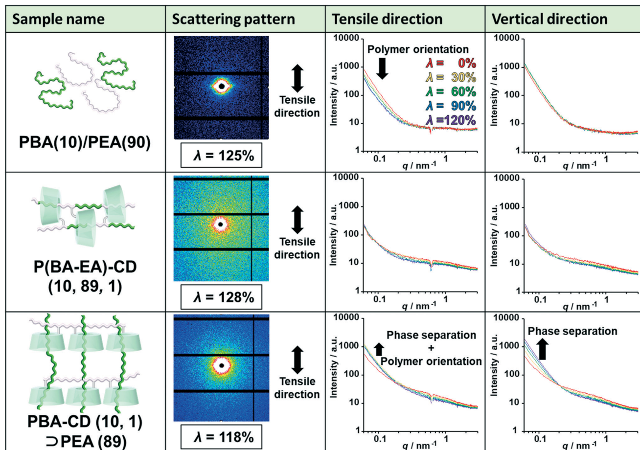
Fig. 5 Scattering patterns of PBA(10)/PEA(90) with 125% strain, P(BA-EA)-CD (10, 89, 1) with 128% strain, and PBA-CD (10, 1)>PEA (89) with 118% strain. SAXS profiles of PBA(10)/PEA(90), P(BA-EA)-CD (10, 89, 1), and PBA-CD (10, 1)>PEA (89) with \lambda strains ( \lambda = 0\% : red line, \lambda = 30\% : yellow line, \lambda = 60\% : green line, \lambda = 90\% : blue line, and \lambda = 120\% : purple line) in the tensile and vertical directions.
