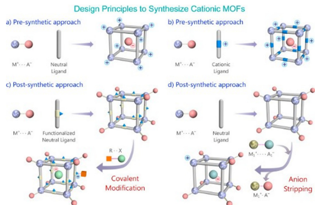
Fig. 5 Schematic representation of routes to build a cationic MOF via pre- and post-synthetic approach. Reproduced with permission from ref. 95.
