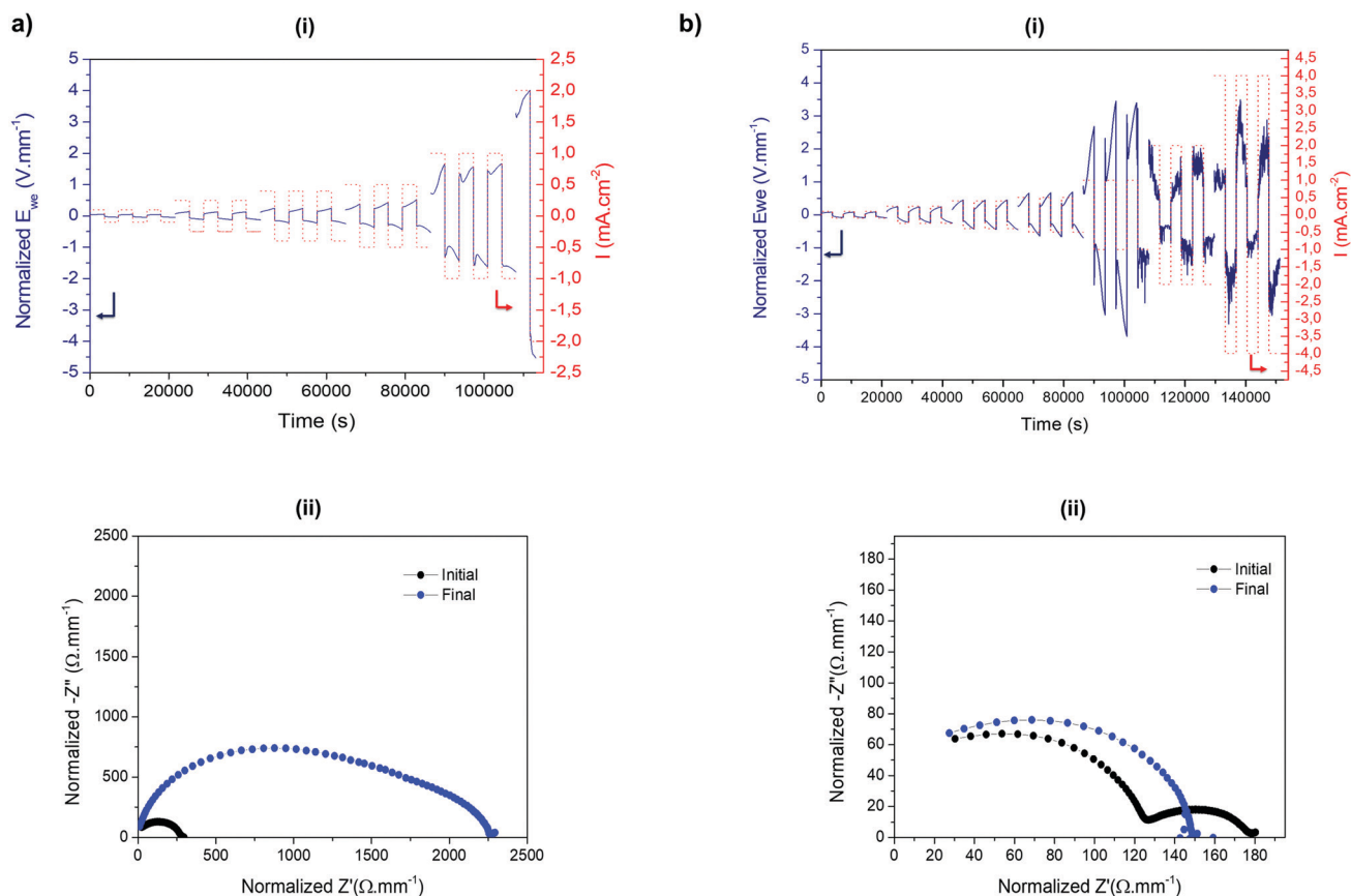
Fig. 8 Galvanostatic cycling with increased current densities for (a) Li|SEIPE|Li and (b) Li|HSIPE-26|Li. (i) Voltage profiles at different current densities. (ii) EIS spectra before and after galvanostatic cycling.
