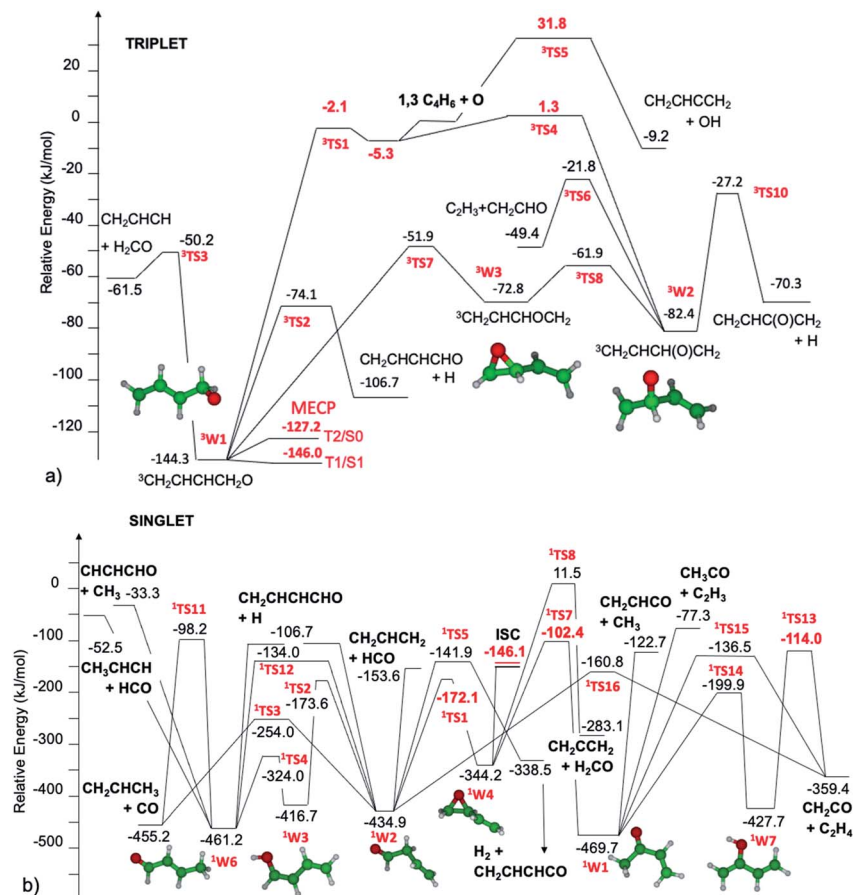
Fig. 1 Schematic representation of the O(^3P) + 1,3-butadiene triplet (a) and singlet (b) potential energy surfaces. Relative energies (kJ mol ^{-1} , 0 K) computed at the CCSD(T)/CBS and CASPT2/aug-cc-pVTZ levels (in red) on \omega B97X-D/aug-cc-pVTZ level structures.
