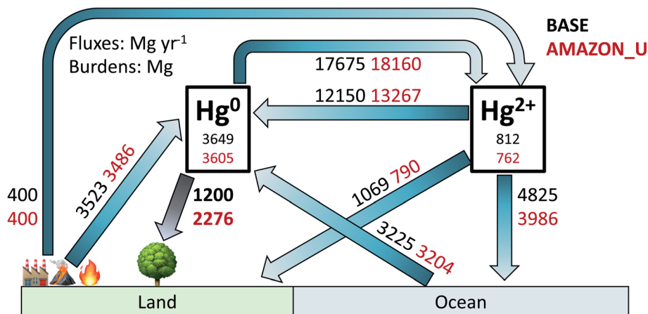
Fig. 6 Atmospheric Hg budget for BASE and AMAZON_U simulations for year 2015. Atmospheric burdens are listed in units Mg and fluxes in Mg per year. The Hg^{2+} burden and fluxes include both gaseous and particulate Hg^{2+} .
