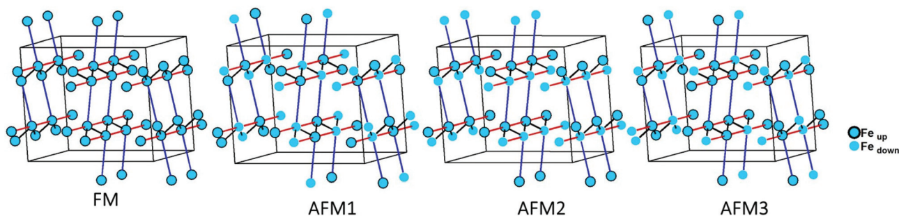
Fig. 4 Different magnetic configurations of Ba_5Fe_2In_4Zn_1S_{15} used in the DFT+U calculations; J_1 , J_2 and J_3 are represented in black, red and blue, respectively.
