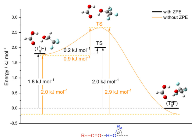
Fig. 5 Energy profile calculated at B3LYP-D3(BJ)/def2QZVP level for the isomerism of the metastable (T_g^t F) complex on the left to the global minimum (T_g^g F) structure on the right (lone pair switch) along the hinge angle. Shown with and without zero-point vibrational energy.
