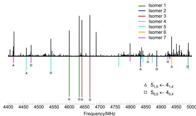
Fig. 2 Section of the rotational spectrum of limonene–(H 2 O) 2 predicted at a rotational temperature of 1 K, showing the 5 0,5 ← 4 0,4 and 5 1,5 ← 4 1,4 rotational transitions for all observed isomers. Upper trace shows the experimental spectrum, lower trace shows the simulated spectrum using the experimentally determined rotational constants.
